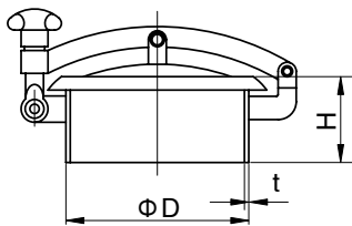
圆型人孔盖 (非压力型) Circular type manhole cover (without pressure)
