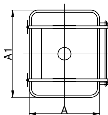
长方形人孔盖 (压力型) Square type manhole cover (with pressure)
